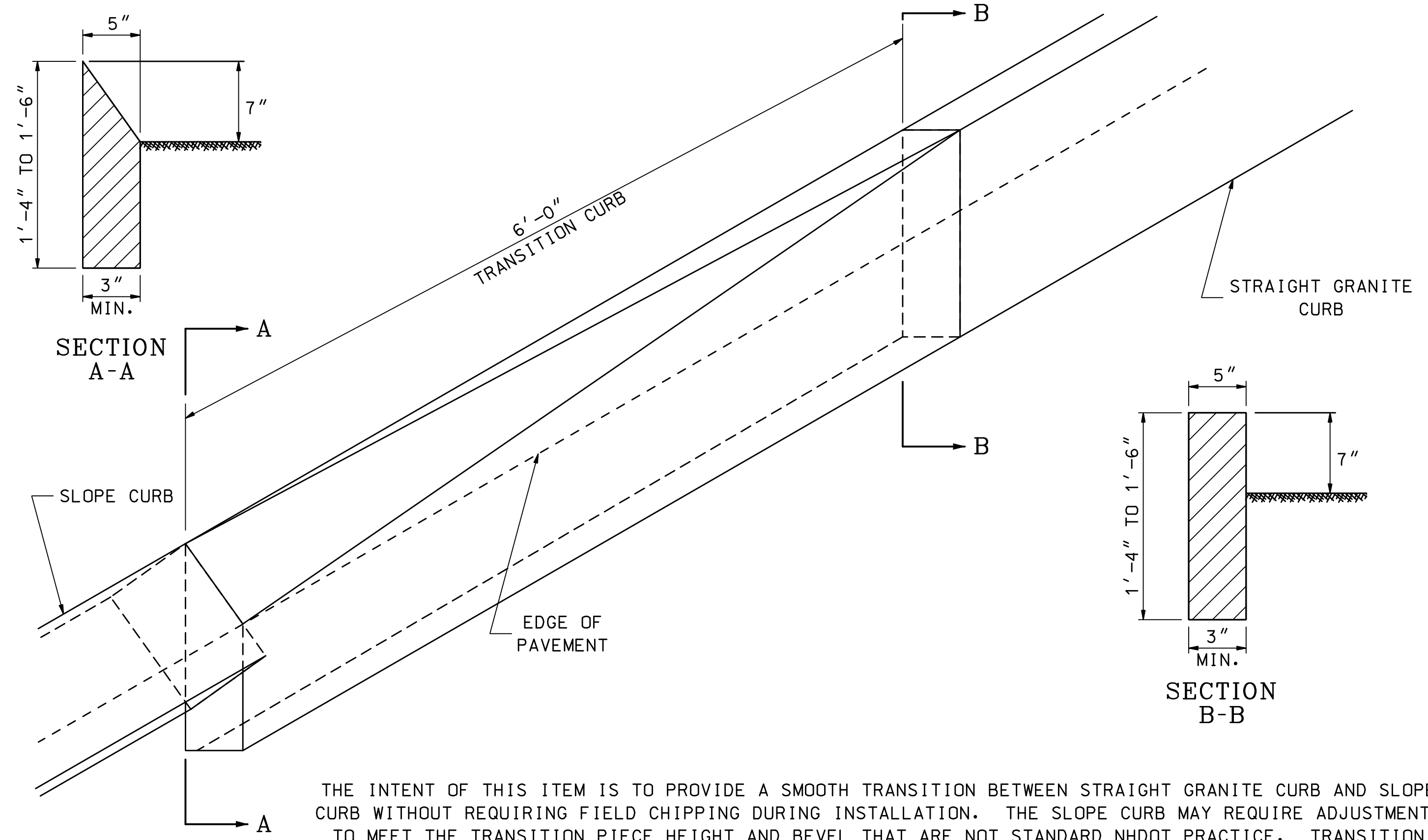
STRAIGHT TO SLOPE CURB TRANSITION
