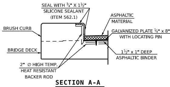
ASPHALTIC PLUG EXPANSION JOINT (F) ITEM 559.4 (CURB DETAIL)
