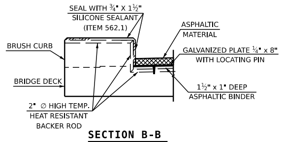
ASPHALTIC PLUG EXPANSION JOINT (F) ITEM 559.4 (U-BACK WINGWALL CURB DETAIL)
