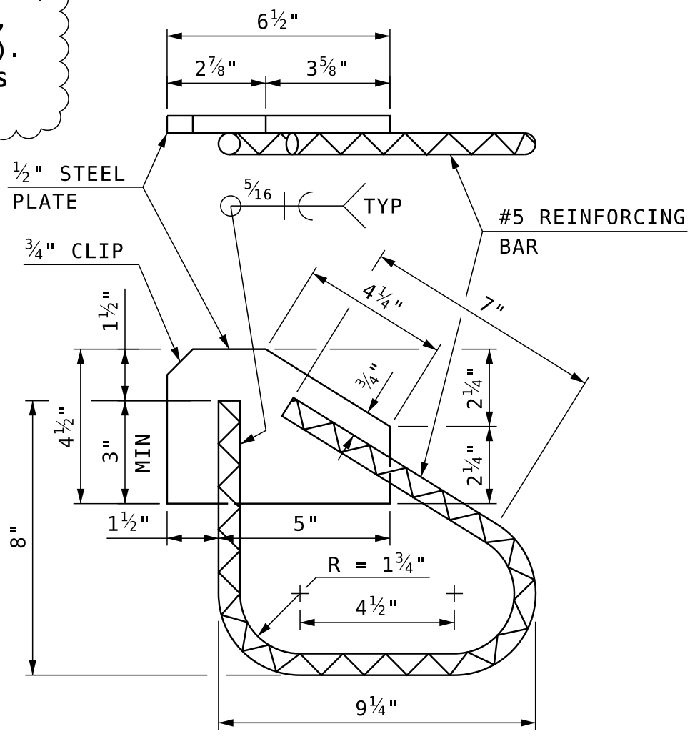
ANCHOR DETAIL (90° CROSSING) SCALE: 3" = 1'-0"
