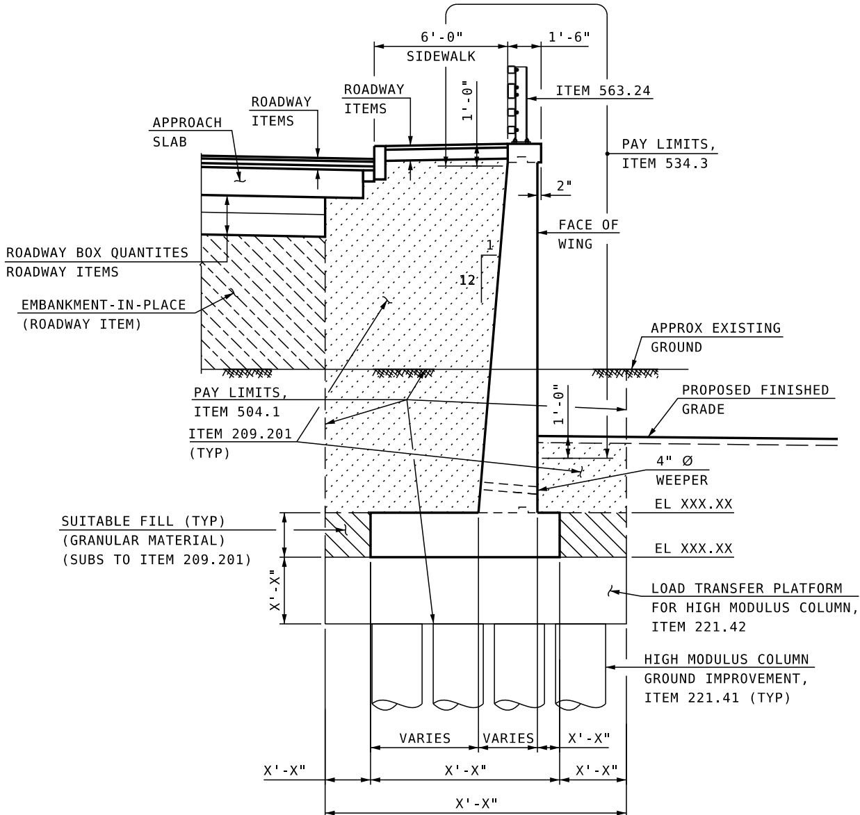
U-BACK WING SECTION WITH SIDEWALK
