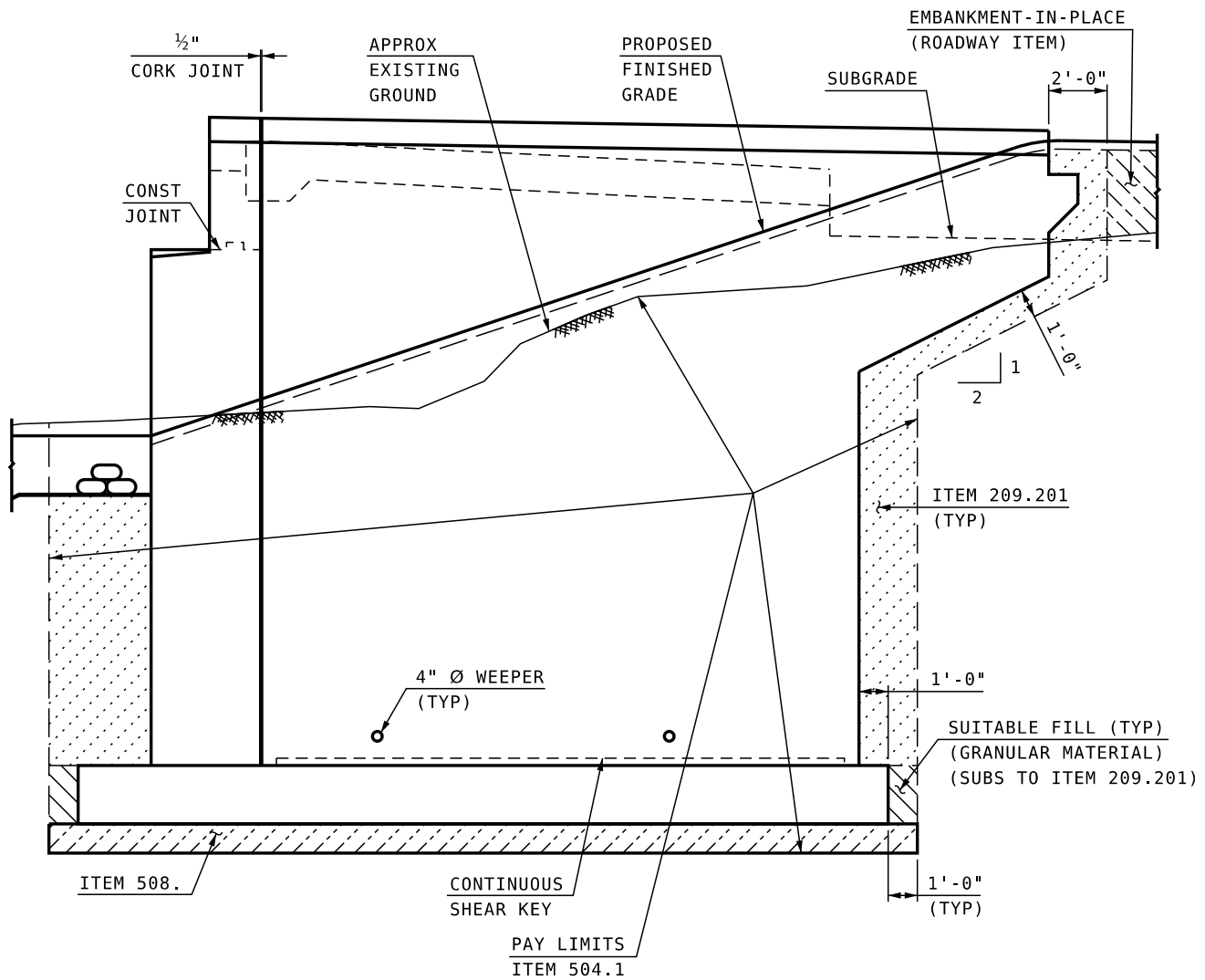
U-BACK WING W/ BUTTERFLY ELEVATION
